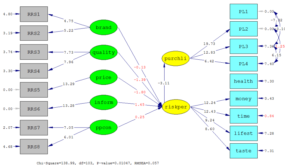
Gambar 3 T-Value Model Struktural Sumber: LISREL 8.70
