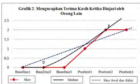
Gambar 6. Trend Analysis Social Stories 2
